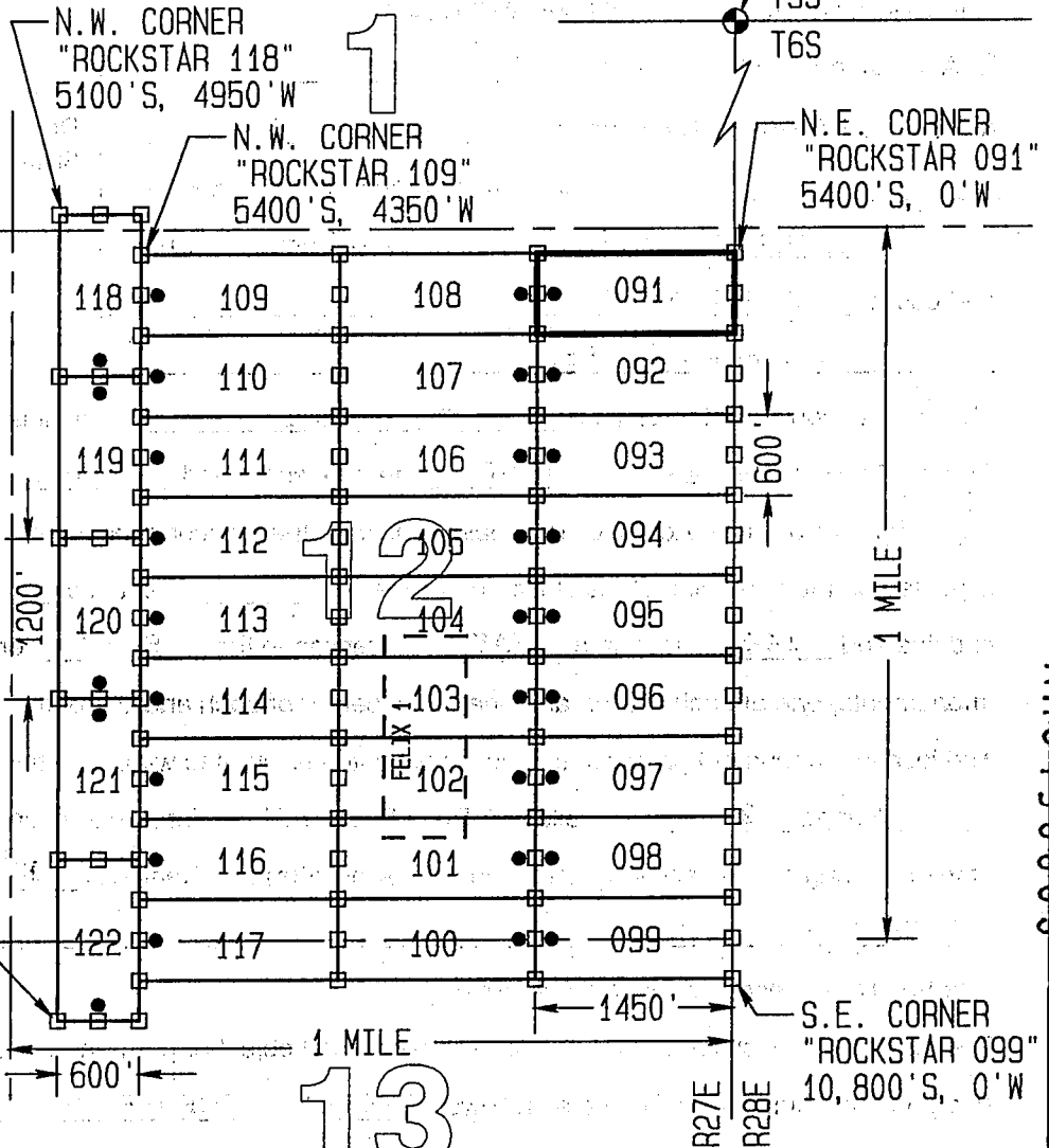
TYPICAL CLAIM DETAIL (NOT TO SCALE) (EXCEPT ROCKSTAR 118-122)
