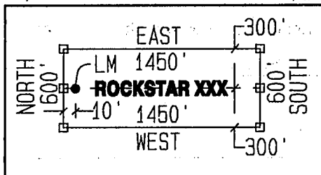
TYPICAL CLAIM DETAIL (NOT TO SCALE) (EXCEPT ROCKSTAR 118-122)
